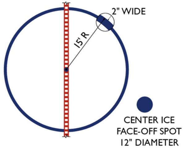
CENTER ICE FACE-OFF SPOT AND CIRCLE DETAIL
