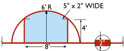
GOAL CREASE DETAIL
